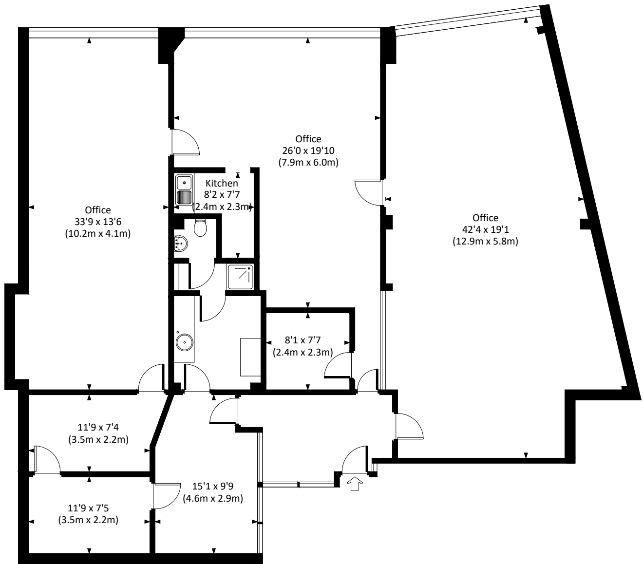
FIRST FLOOR
